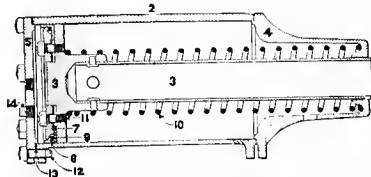
Fig. 1726. TENDER BRAKE-CYLINDER.
